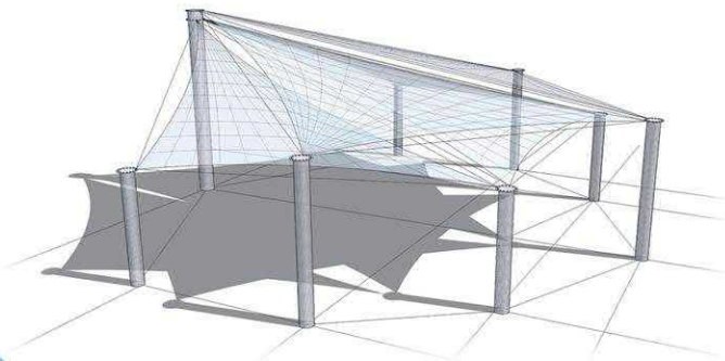
1 Design & Development (D&D) Phase: Conceptual sketch of design
