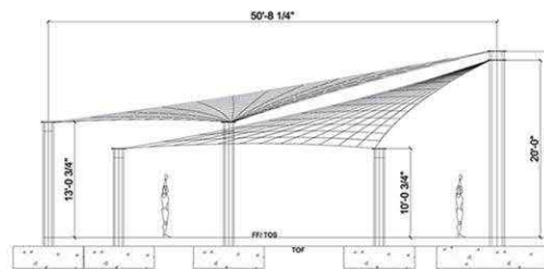
ELEVATION FRONT
