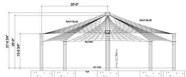
ELEVATION SIDE
