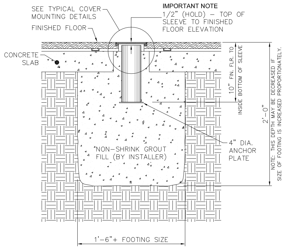
TYPICAL INSTALLATION DETAIL
